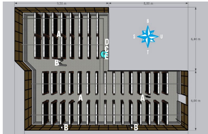
Figure 3. Mushroom Cultivation Chamber Plan
