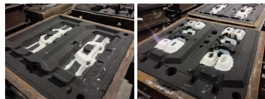
Figure 11. Coating of the first layer in the O3
