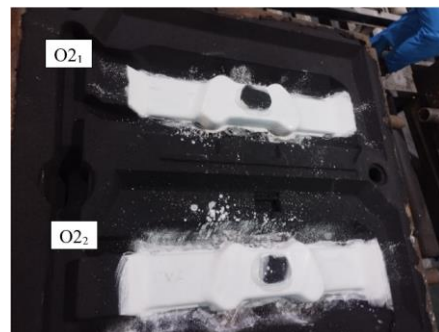
Figure 7. The first layer coating of experimental group O2
