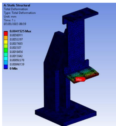
Figure 11. Deformation for Area 2
