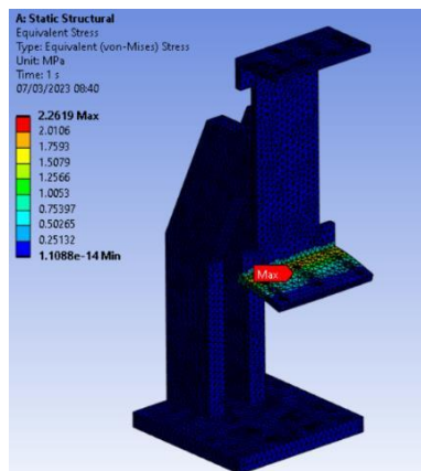
Figure 10. Von Mises Stress Simulation Results for Area 2
