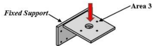
Figure 4. Loading on the Motor Mount Frame
