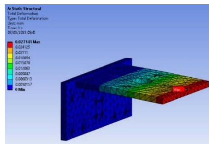
Figure 15. Deformation for Area 3
