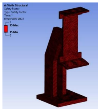
Figure 12. Safety Factor for Area 2
