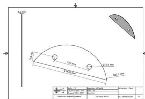
Figure 5. Blade design
