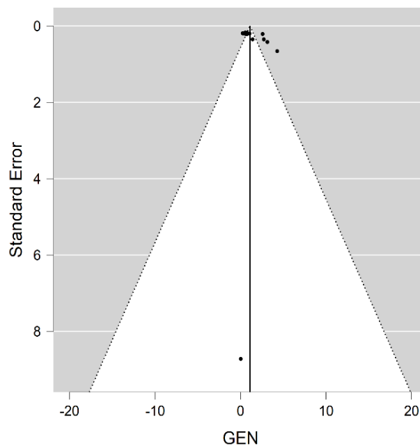
Gambar 2. Funnel Plot
