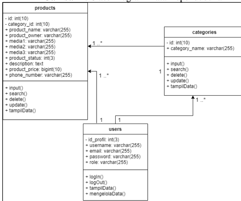
Gambar 5. Class Diagram Pasar Online
