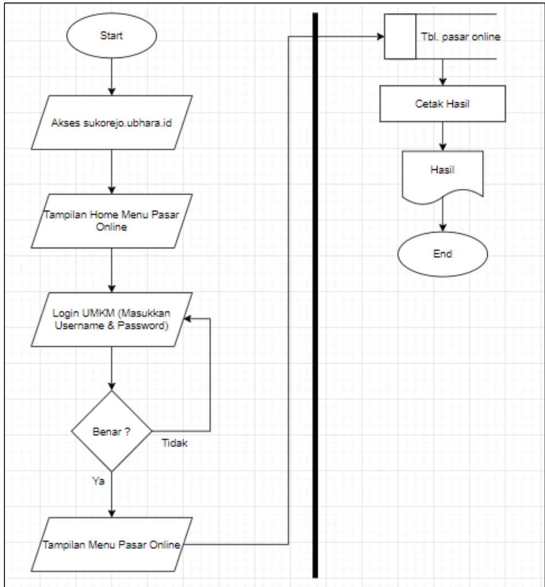
Gambar 3. Flowchart Pasar Online
