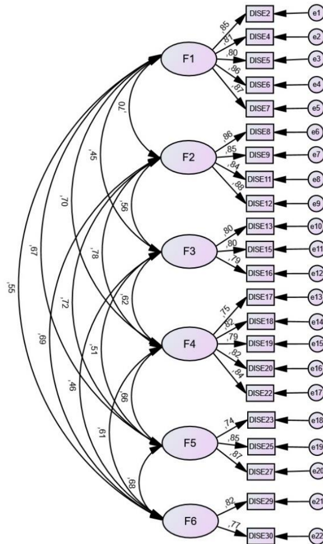
Figure 2. CFA Model
