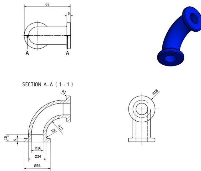
Fig. 1. Design of the intake manifold
