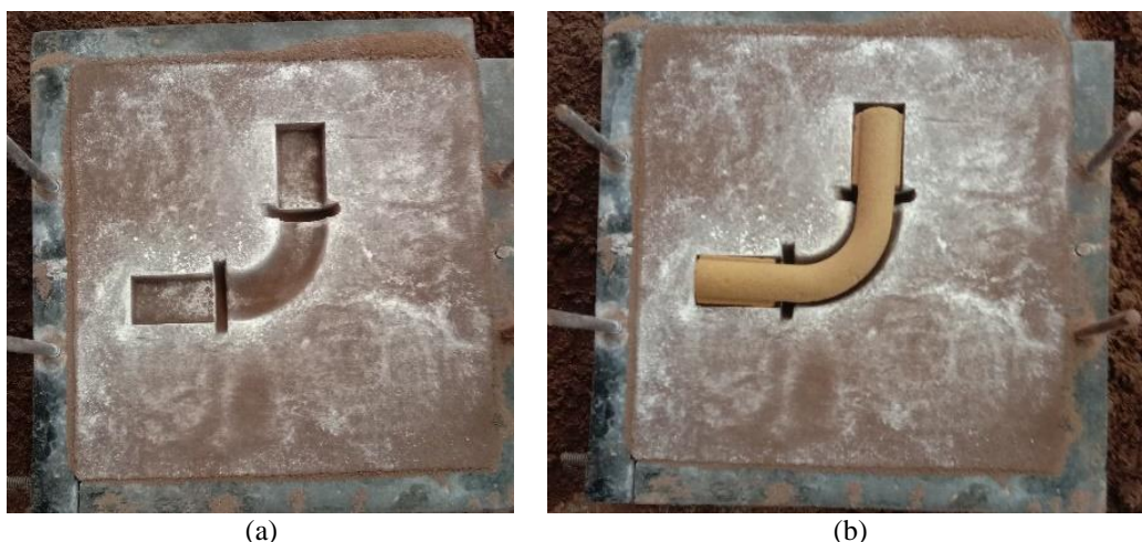
Fig. 10. (a) Sand mold after pattern revised; (b) Placement of sand core after revised
