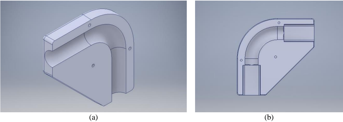
Fig. 7. Revision of core box patterns on (a) Cope; and (b) Drag.
