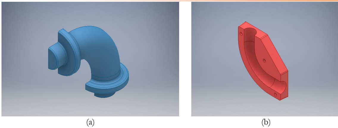
Fig. 3. Pattern design of (a) Intake manifold; (b) Core box
