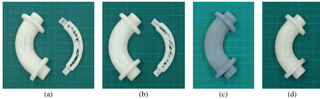
Fig. 1. Pattern printout results of (a) Trial 1; (b) Trial 2; (c) Trial 3; (d) Trial 4
