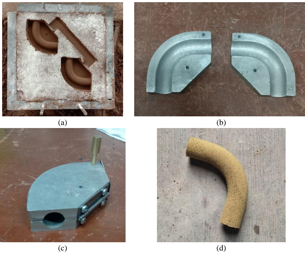
Fig. 4. (a) Sand moulding of a core box; (b) Core box castings results; (c) Final core box; (d) Sand core
