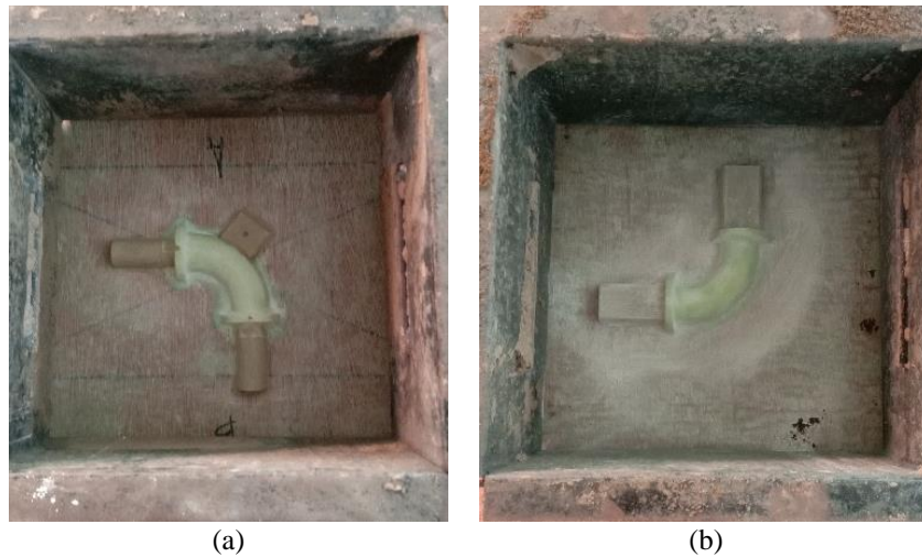
Fig. 8. Pattern revision on (a) Cope; and (b) Drag
