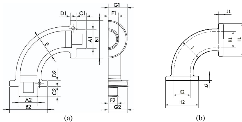
Fig. 2. Measurement section on (a) Pattern; (b) Casting product.
