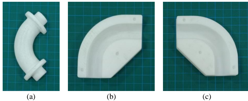
Fig. 2. (a) Printout of mirror pattern of the fourth trial; (b,c) Printout of the core box
