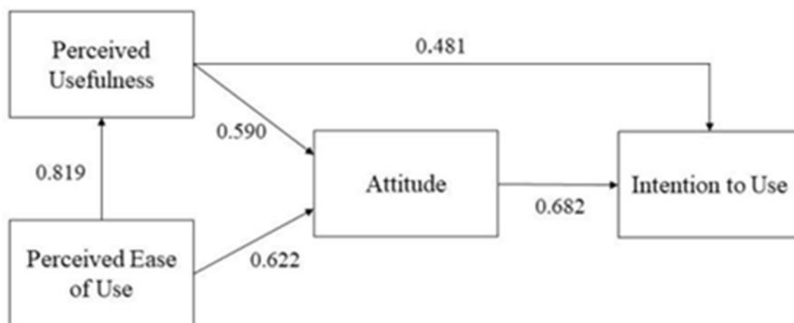
Figure 7. TAM correlation relationship
