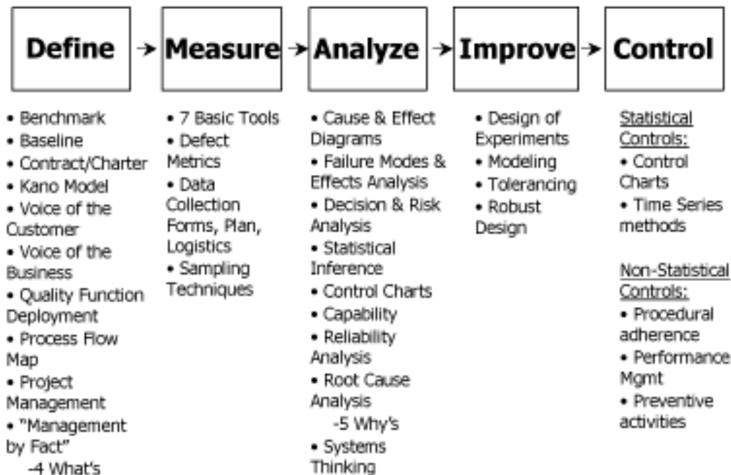
Figure 1 : Six Sigma Improvement Framework and Toolkit (Jeannine Sivi, 2001)
