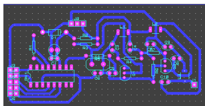
Gambar 5. Layout PCB
