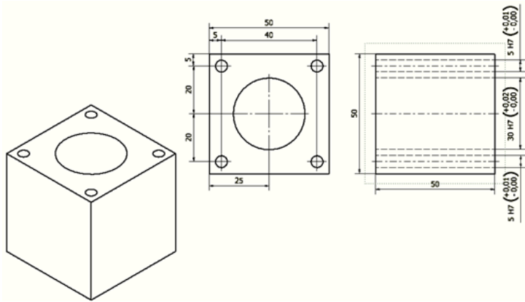
Gambar 5. Block Cylinder Panas/Dingin
