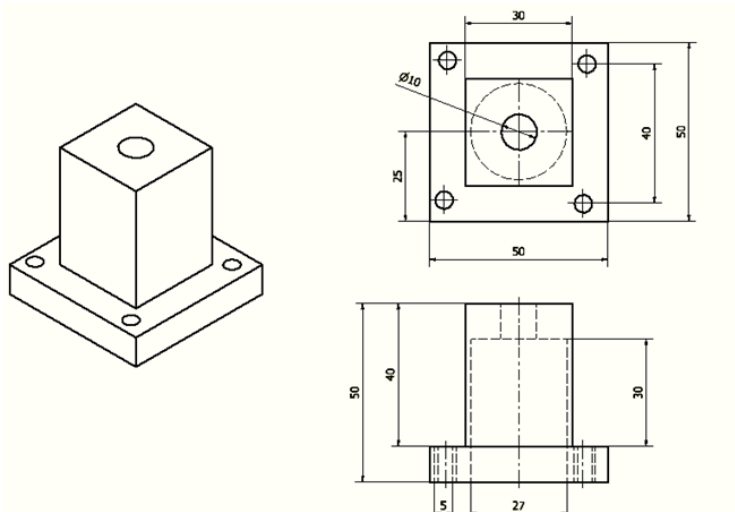
Gambar 6. Cylinder Head Panas
