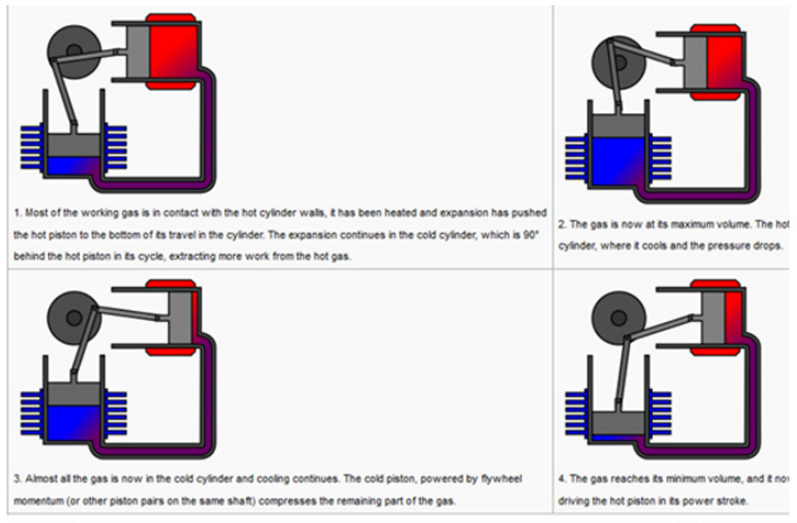
Gambar 2. Prinsip Kerja (Sumber: http://en.wikipedia.org/wiki/stirling_engine )
