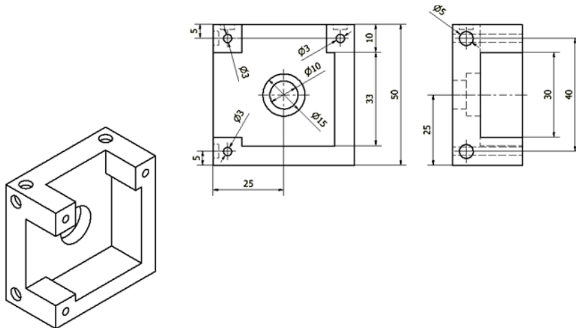
Gambar 4. Crankcase
