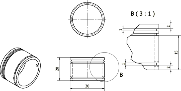
Gambar 8. Piston Dingin
