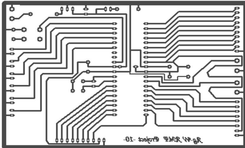
Gambar 7 Layout PCB
