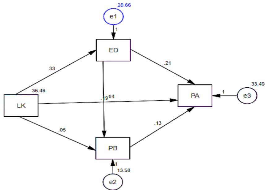
Gambar 1. Diagram Jalur (Path)
